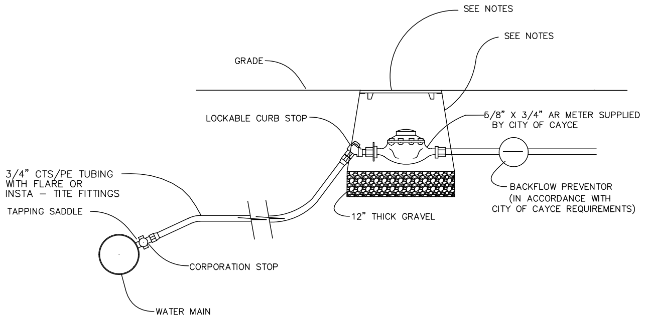
WATER SERVICE DETAIL NOT TO SCALE
